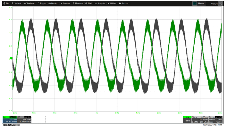
Figure 7. Measured motor phase currents powering a vacuum cleaner motor operating at 50 krpm
