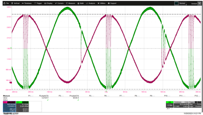
Figure 4. Phase current and current sense signals. Note that the voltage threshold is positive, but the kelvin connections on the shunt resistor make the overcurrent circuit active at negative current values. As measured by the cursors, the overcurrent threshold is set at -32 A
